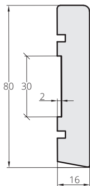
moulding width 80 mm
