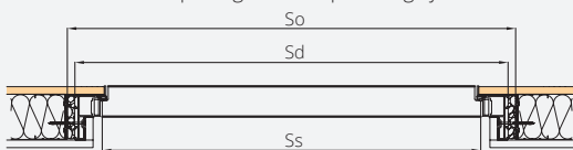
Inward-opening door for panelling system
