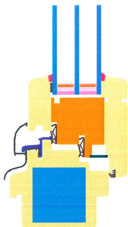
Calculation model
